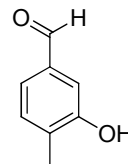
3-hydroxy-4-methylbenzaldehyde
