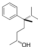
(2 R ,5 S )-5,6-dimethyl-5-phenylheptan-2-ol
