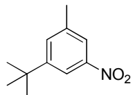
3-( tert -butyl)-5-nitrotoluene
