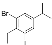
1-bromo-2-ethyl-3-iodo-5-isopropylbenzene
