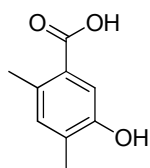
5-hydroxy-2,4-dimethylbenzoic acid
