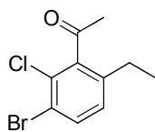
3-bromo-2-chloro-6-ethylacetophenone
